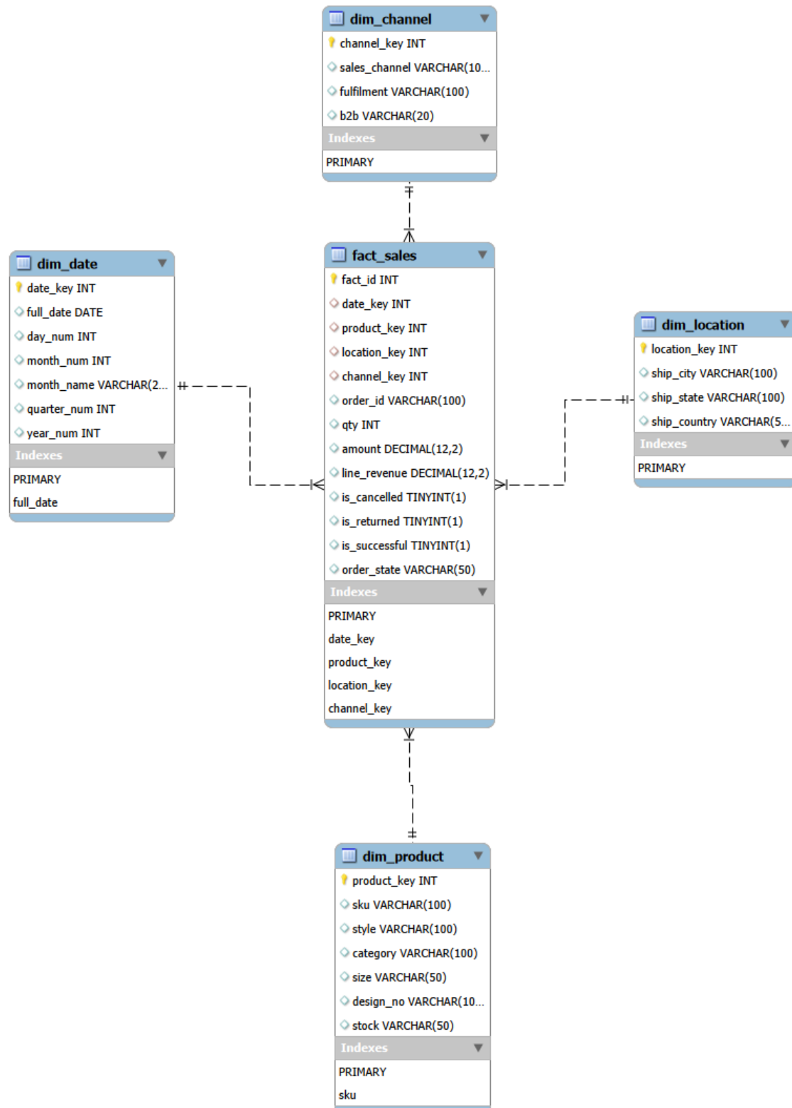
ERD diagram showing DIMENSION Tables and the relationships between them.
